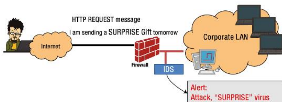
Figure. Signature based detection
